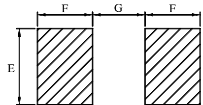
Land Pattern
